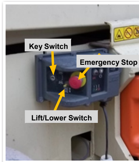
Lower Controls for ES Series
